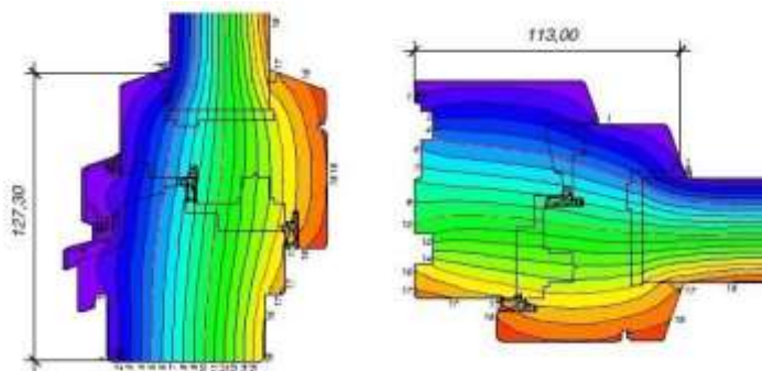
Simulation IV92 acc ISO 10077/2 and 10077/1 - value of frame U_f=0,94 and with aluminium waterbar U_f=1,10 W/m 2 K
